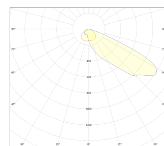
Asimetrik Lens / Asymmetric Lens
