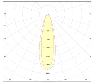
30 Derece Lens / 30 Degree Lens
