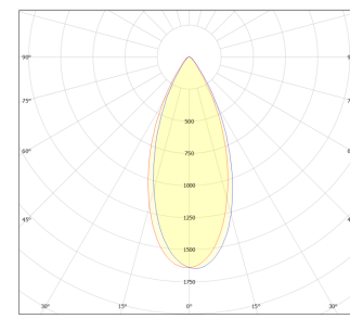
45 Derece Lens / 45 Degree Lens
