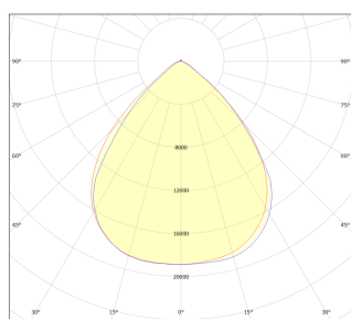
90 Derece Lens / 90 Degree Lens
