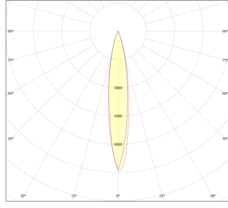
15 Derece Lens / 15 Degree Lens
